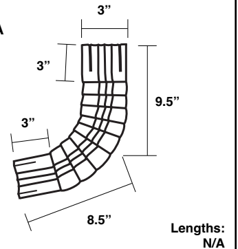
Lock-Seam Downspout - Center
