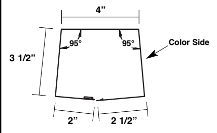
Lock-Seam Downspout - Center
