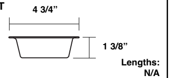
3" x 4" Downspout Elbow A-Style BBPELA
