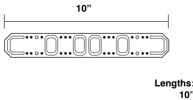
Lock-Seam Downspout Outlet - Standard
