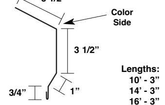
Shingle Rake Trim (P-SRT)
