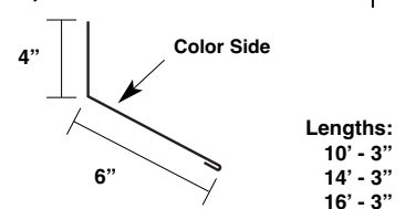
High Side Tie-In* (P-SWF)
