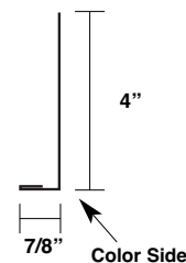
Angle Trim 7/8" x 4" MTA4
