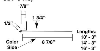
Overhead Door Flashing 6 1/2" (P-JF-B-6 1/2)
