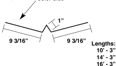
Rake and Gable Trim (P-RF)
