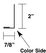
Angle Trim 7/8" x 2" MTA2
