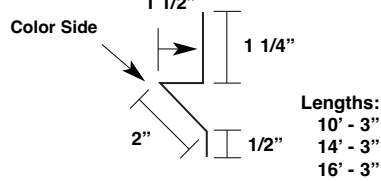
Mini-Outside Corner (P-MOC)
