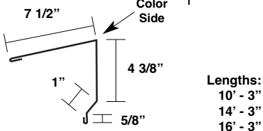
High Side Trim* P-HSE
