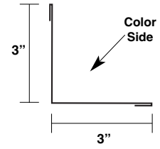
Inside Angle Trim P-IA
