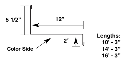
Eave Flashing* (P-EF)*
