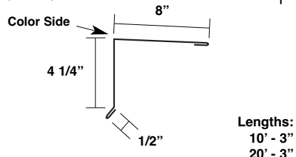
Ridge Cap* (R-RC-13)
