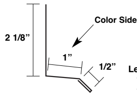
Base Drip P-DF
