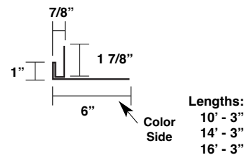
Overhead Door Flashing 8 7/8" (P-JF-B-8 7/8)
